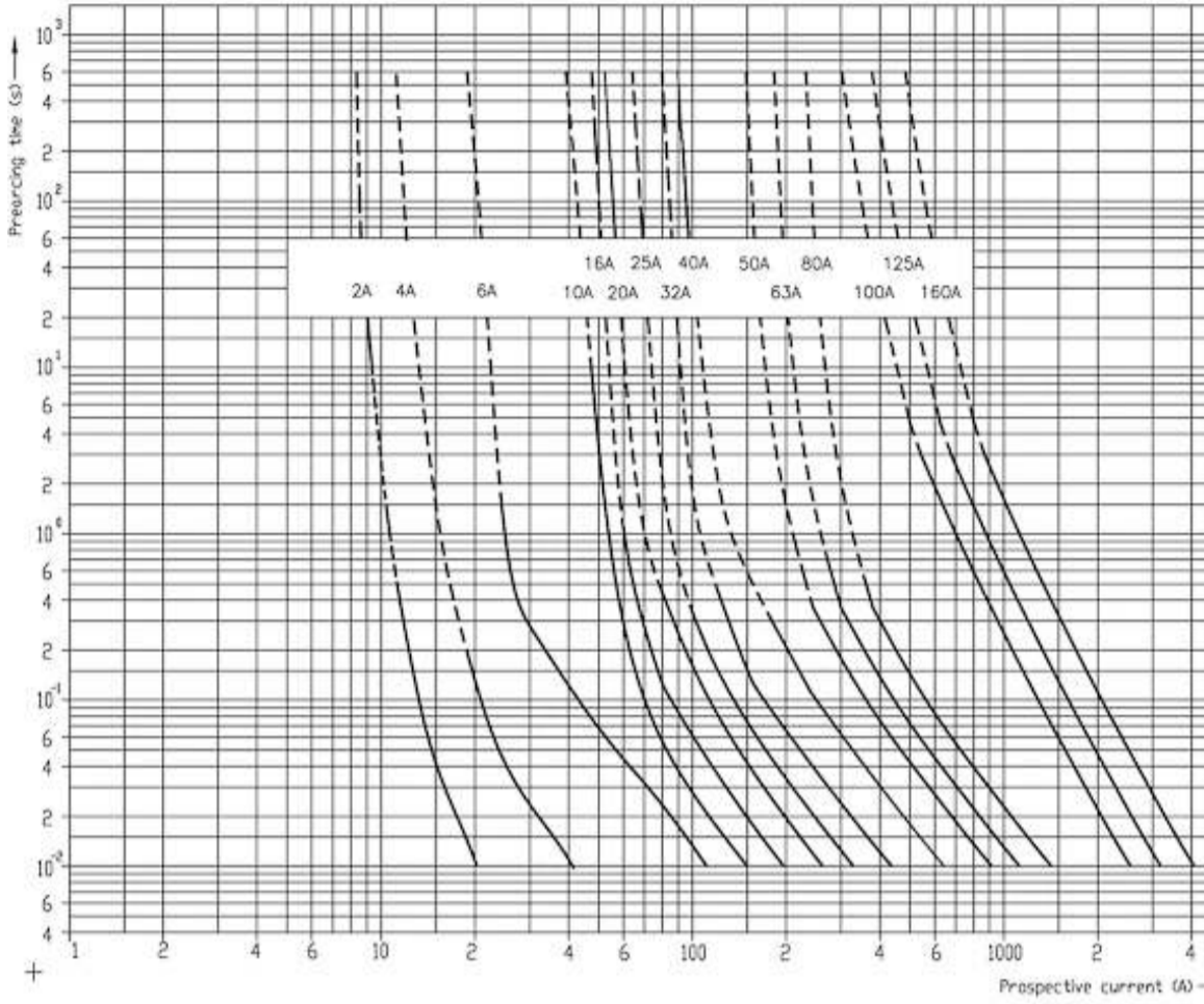
Time-current characteristics for VV-thermo fuse links
