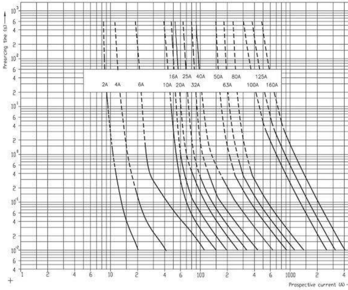
Time-current characteristics for W-thermo fuse links
