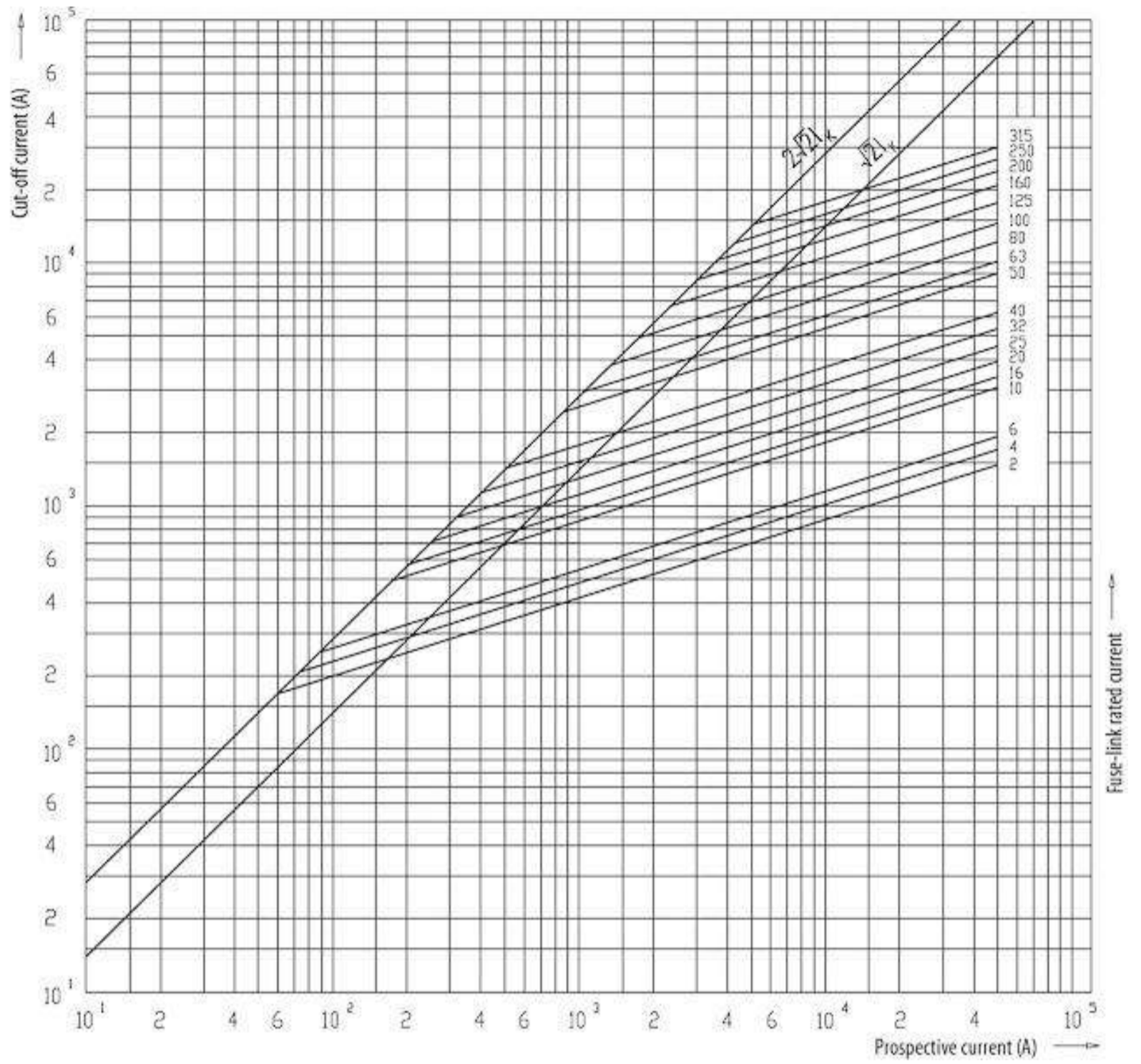
Cut-off current diagram for VV-Thermo fuse links
