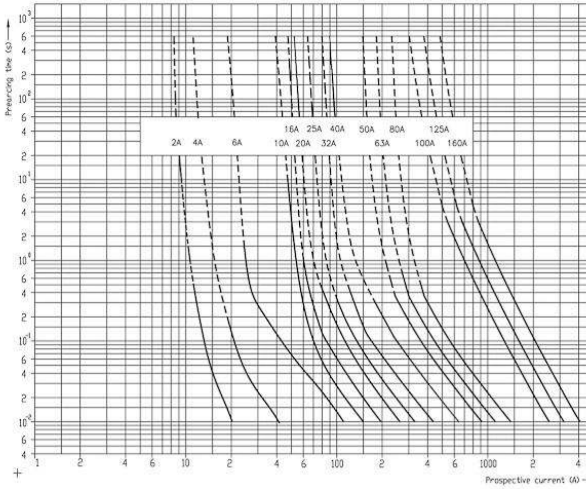
Time-current characteristics for W-thermo fuse links
