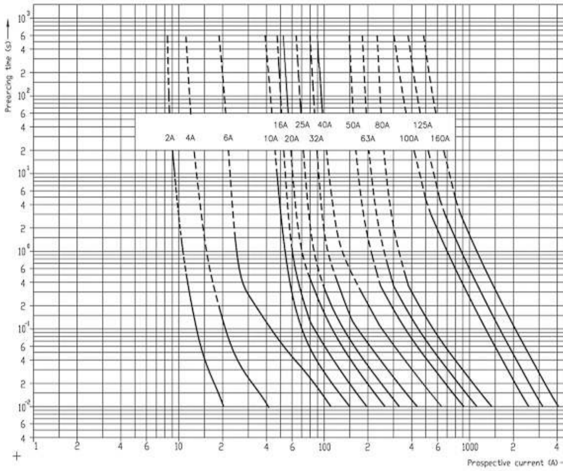
Time-current characteristics for VV-thermo fuse links
